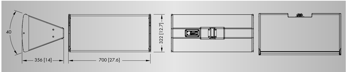
ALi90 cabinet dimensions in mm [inch]
