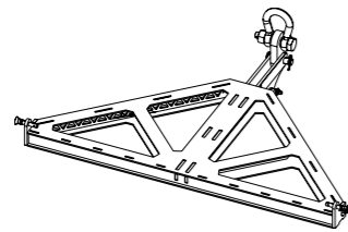
Z5725 KSL Compression frame
