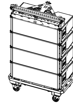
E7802 4 x KSL8/KSL12 Touring cart Loaded in Compression mode with mounted vKSL Flying frame and KSL Load beam
