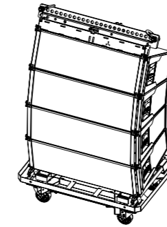
E7495 4 x KSL8/KSL12 Touring cart Loaded in Tension mode with mounted KSL Flying frame and KSL Load beam
