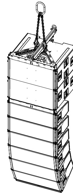
KSL-SUB/ KSL8/12 Mixed array Compression mode - Front
