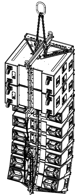
KSL-SUB/ KSL8/12 Mixed array Compression mode - Rear
