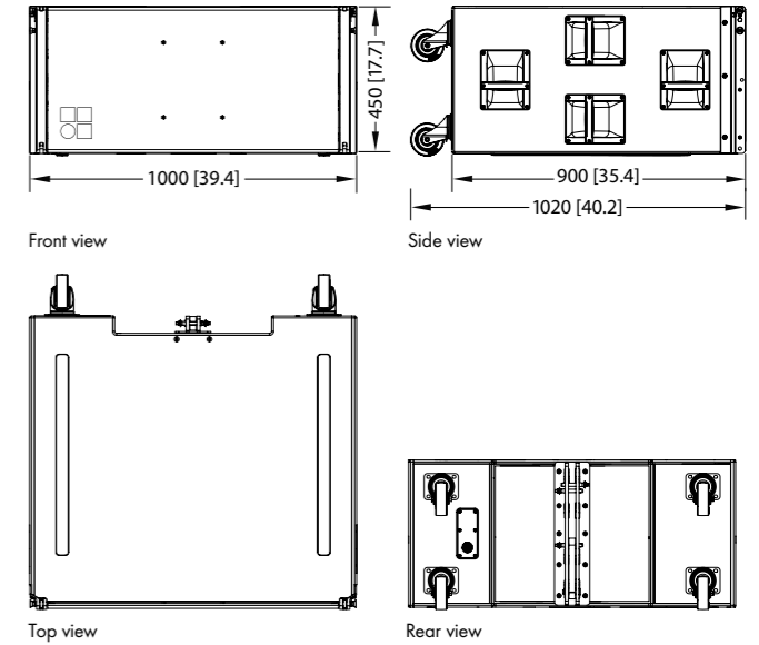
KSL-SUB/KSL-GSUB cabinet dimensions in mm [inch]
