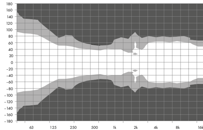
KSL12 horizontal dispersion characteristics 3
