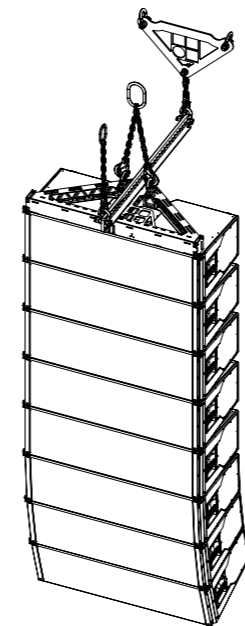
KSL8/12 Line array 8-deep Tension mode - Front
