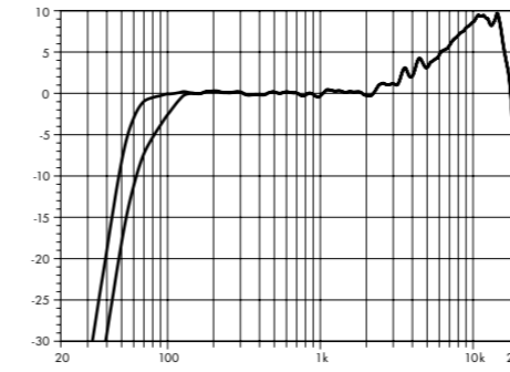
KSL8 frequency response, standard and CUT modes 1
