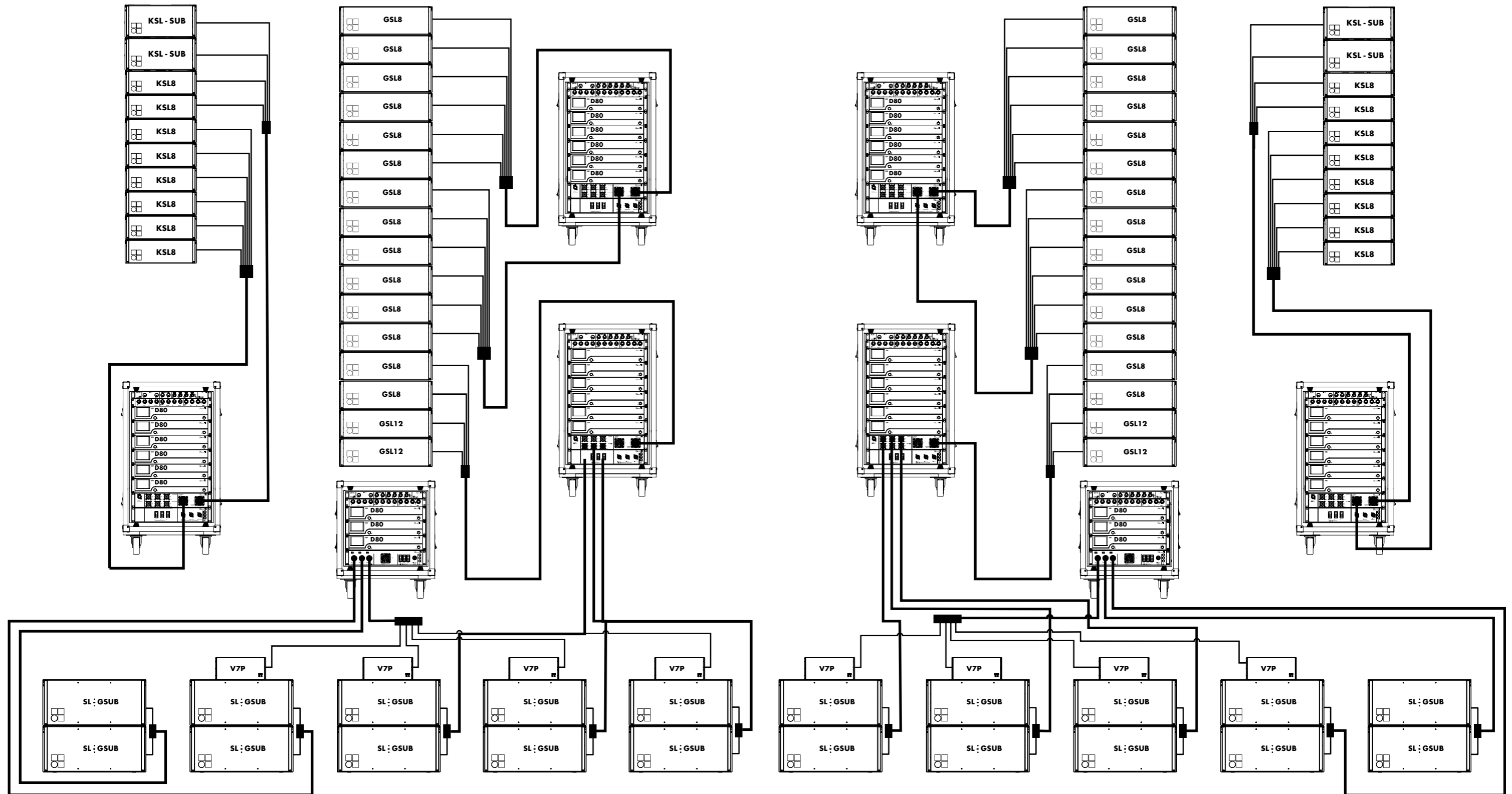
SL-Series festival configuration comprising GSL8/GSL12 mains, KSL-SUB/KSL8 outfills and V7P frontfills along with ground stacked SL-GSUB with 6 x D80 and 3 x D80 Touring racks
