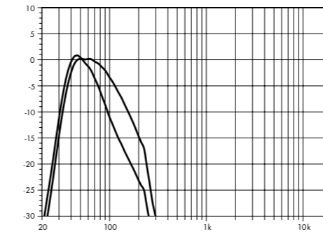
KSL-SUB/KSL-GSUB frequency response, standard and INFRA modes
