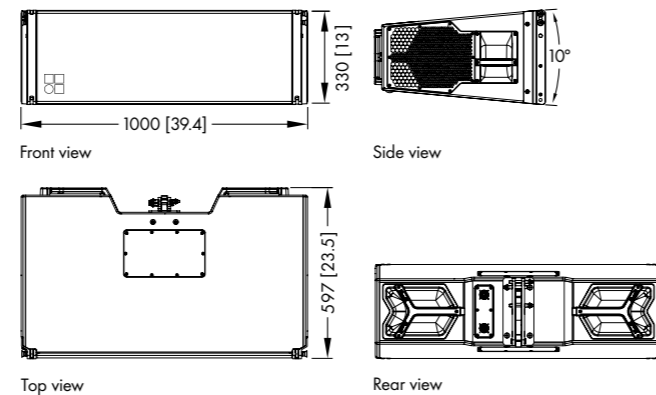
KSL8/KSL12 cabinet dimensions in mm [inch]
