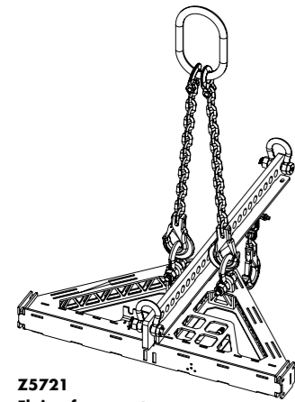
Z5721 Flying frame set
