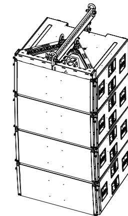
KSL-SUB column 4-deep 2° splay Front
