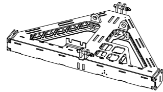
Z5722 KSL Flying frame
