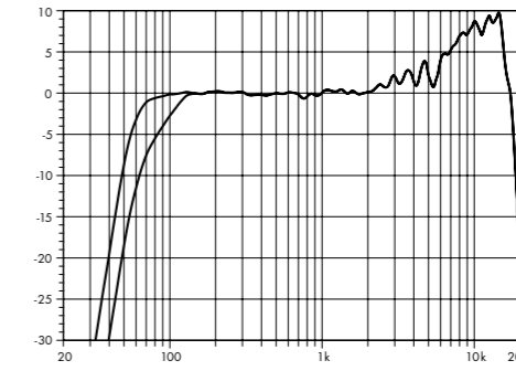
KSL12 frequency response, standard and CUT modes 1
