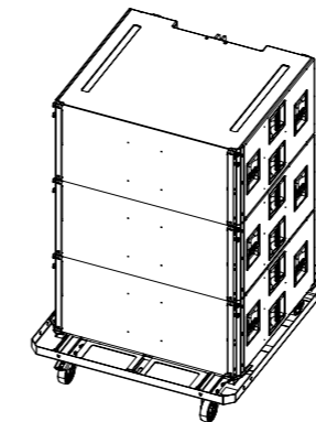
E7804 KSL-SUB/KSL-GSUB Touring cart
