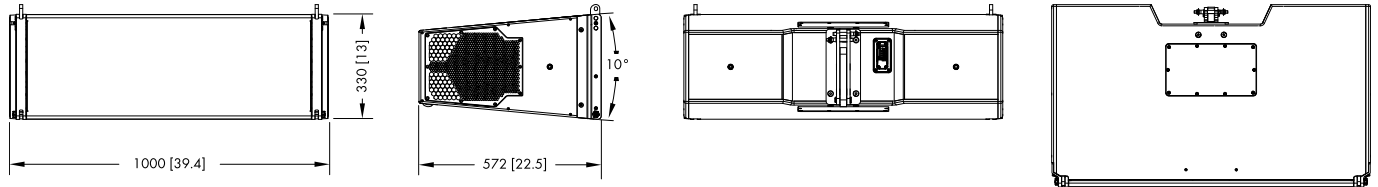
KSLi12 cabinet dimensions in mm [inch]
