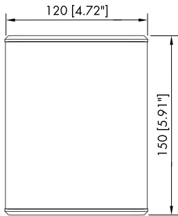
4S cabinet dimensions in mm [inch]
