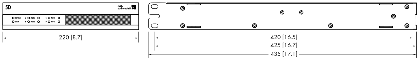
5D dimension in mm [inch]
