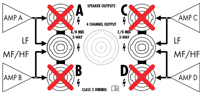
2 x modo 2-Way Active
