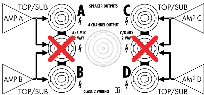
2 x modo Dual Channel
