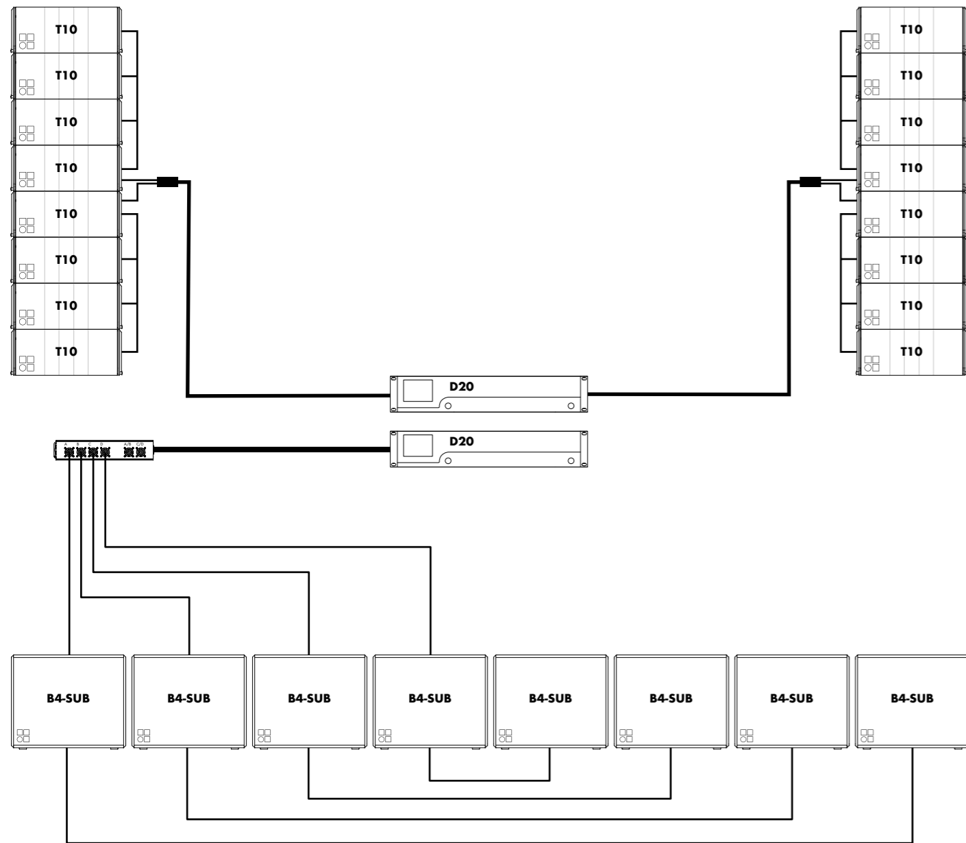
T10 flown line arrays in left/right configuration and ground stacked B4-SUB array with D20 amplifiers in Dual Channel mode 1
