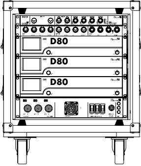
Z5570/Z5571.xxx OUT: LKA25F/3 x NL8
