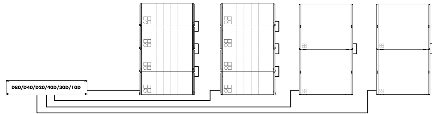
D80/D40/D20/40D/30D/10D amplifier in Dual Channel mode for T10, Ti10L, Ti10P, T-SUB, Ti-SUB and B4-SUB 1
