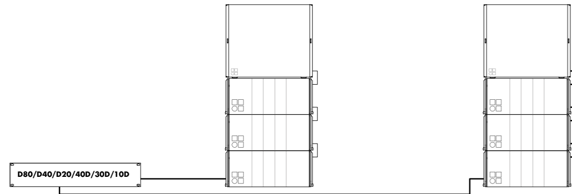
D80/D40/D20/40D/30D/10D amplifier in Mix TOP/SUB mode for T10, Ti10L, Ti10P, T-SUB, Ti-SUB and B4-SUB 1
