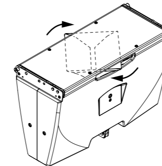
Rotating horn
